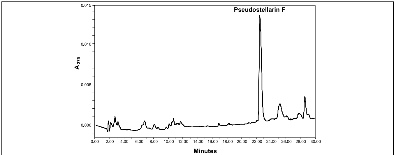
Fig. 5. HPLC characterization of in vitro cyclized pseudostellarin F. Chromatogram of the high salt eluate from a chitin affinity column after overnight incubation of proteins purified following bacterial expression of a SICLOPPS construct encoding pseudostellarin F. Chromatographic conditions and peak identification are as previously described [21].
